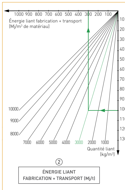
Figure 21 : zone retraitement - Quadrant Energie liant
