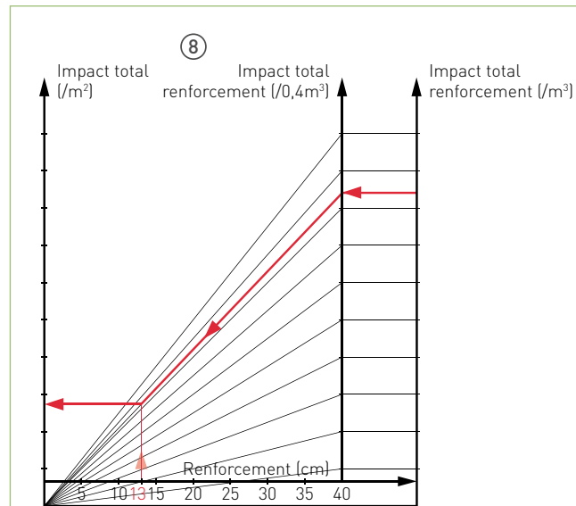
Figure 9 : zone renforcement - Quadrant impact total (/m 3 et /m 2 )
