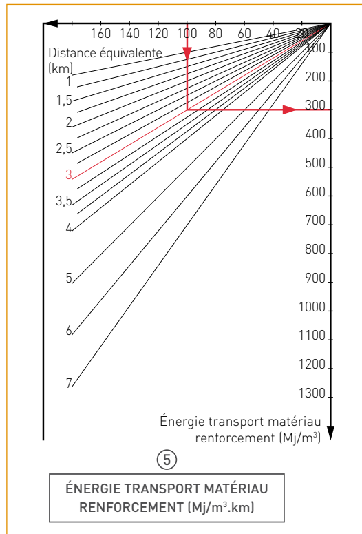
Figure 25: zone renforcement - Quadrant Energie transport matériaux
