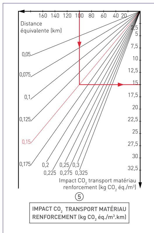
Figure 35 : zone renforcement - Quadrant impact CO 2 transport matériaux
