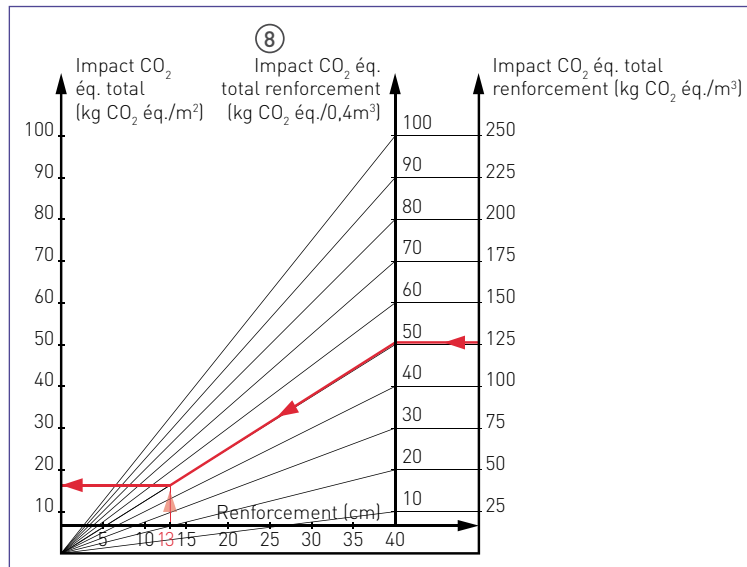
Figure 38 : zone Renforcement - Quadrant impact CO 2 total (kg CO 2 eq./m 3 et kg CO 2 eq./m 2 )
