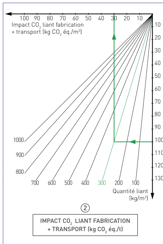
Figure 31 : zone Retraitement - Quadrant impact CO 2 liant
